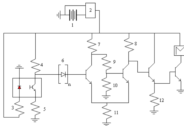
Figure 47: The second control circuit got rid of the op-amps all together, and instead used 4 transistors.
